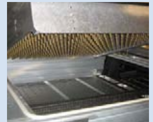
Preheating section in modular design with medium and short-wave emitters and convection heaters
